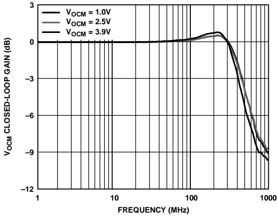
Figure 19. Small Signal Frequency Response for Various V_{OCM}
