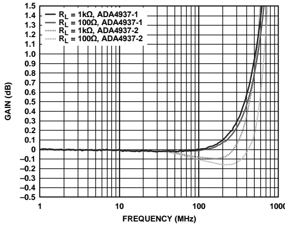
Figure 20. 0.1 dB Flatness Response for Various Loads
